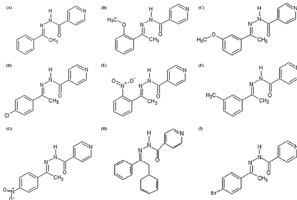
FIG 1 Structural formulas of synthesized isoniazid derivatives N' -[1-phenylethylidene]isonicotinohydrazide (A), N' -[1-(2-methoxyphenyl)ethylidene]isonicotinohydrazide (B), N' -[1-(3-methoxyphenyl)ethylidene]isonicotinohydrazide (C), N' -[1-(4-chlorophenyl)ethylidene]isonicotinohydrazide (D), N' -[1-(2-nitrophenyl)ethylidene]isonicotinohydrazide (E), N' -[1- m -tolylethylidene]isonicotinohydrazide (F), N' -[1-(4-nitrophenyl)ethylidene]isonicotinohydrazide (G), N' -(1,2-diphenylethylidene)-2-isonicotinohydrazide (H), and N' -[1-(4-bromophenyl)ethylidene]isonicotinohydrazide (I).
