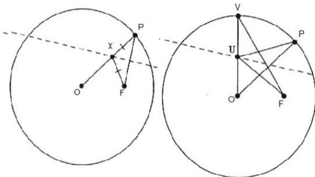
Figura 60: Elipse
