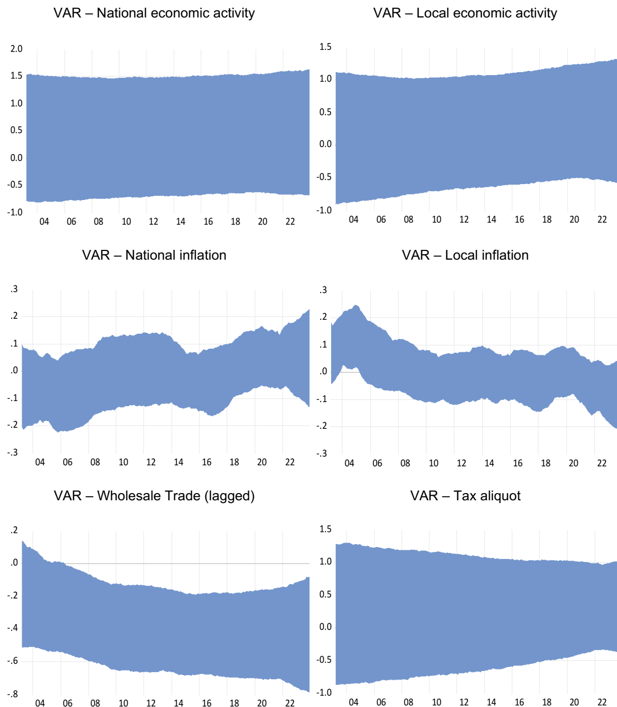
Figure 4 - TVCVAR – Wholesale Trade equation coefficients – median (80% CL)
