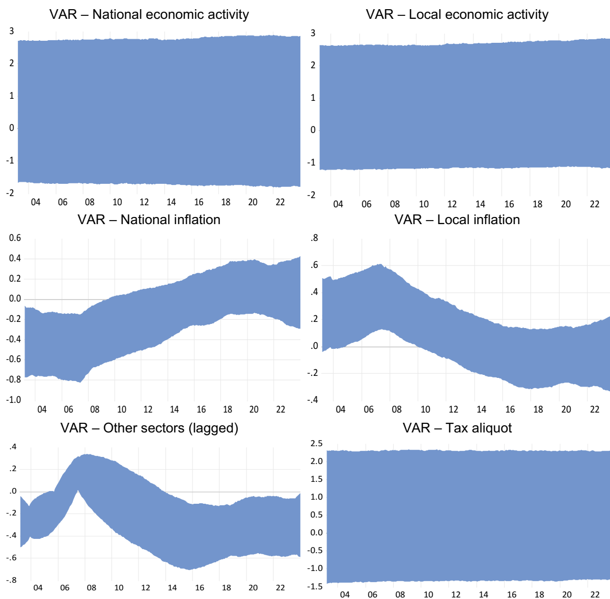
Figure 8 - TVCVAR – Other sectors equation coefficients – median (80% CL)
