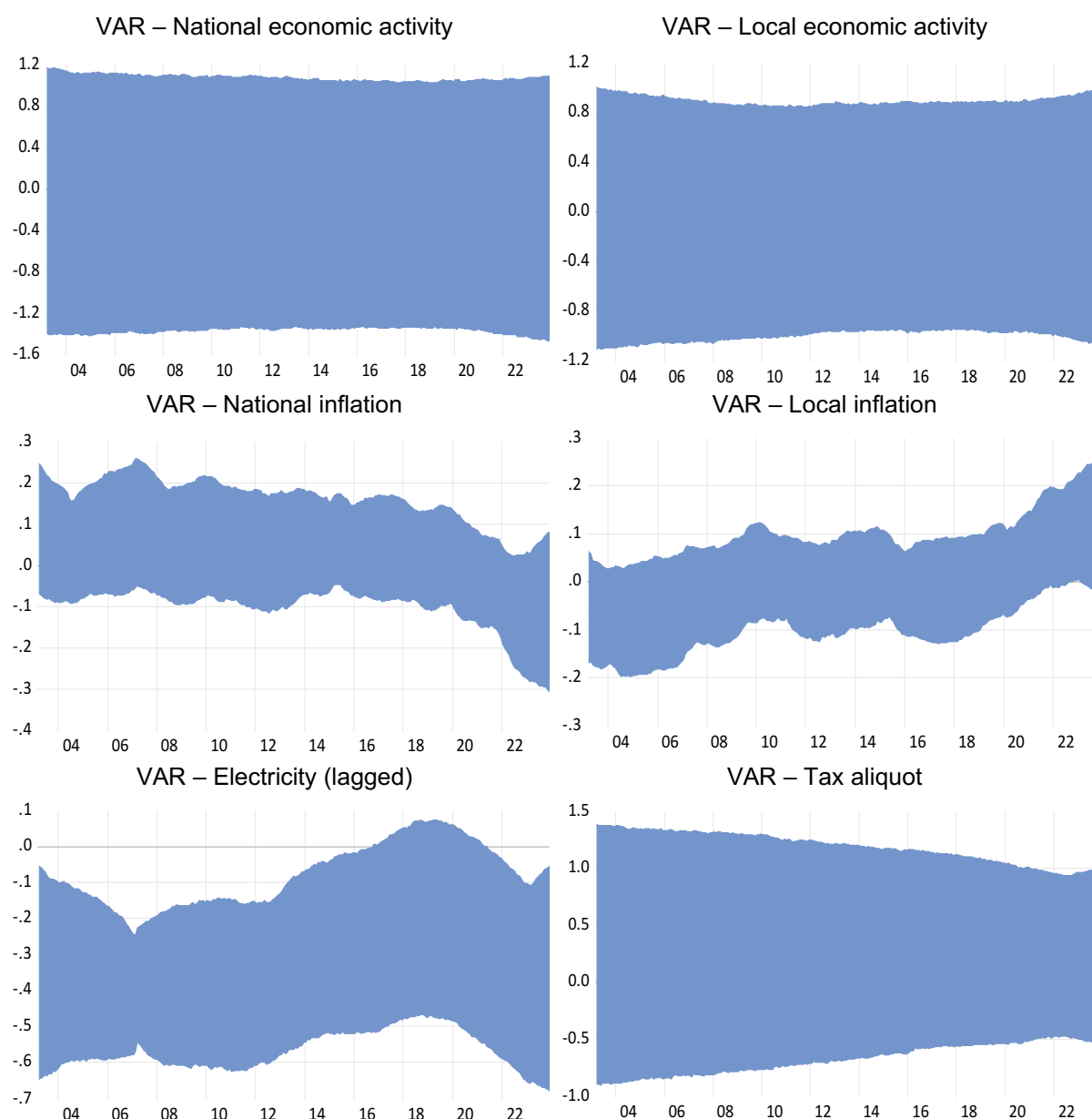
Figure 6 - TVCVAR – Electricity equation coefficients – median (80% CL)
