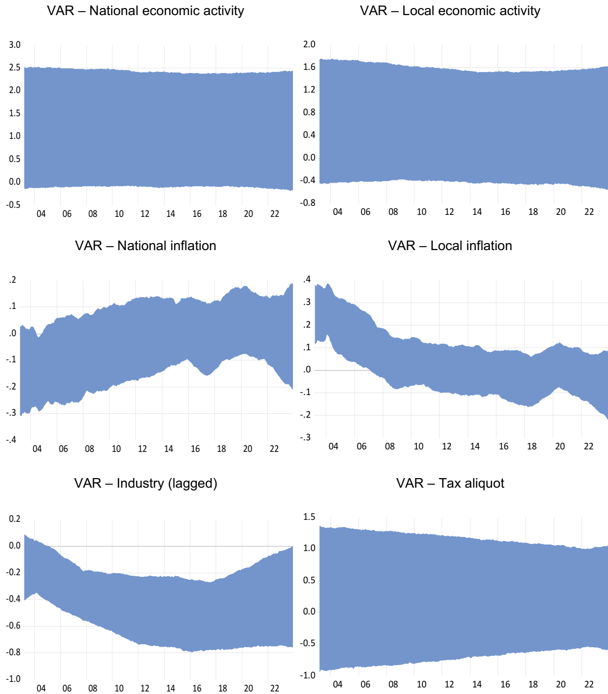
Figure 5 - TVCVAR – Industry equation coefficients – median (80% CL)
