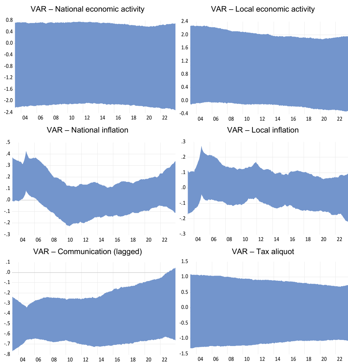
Figure 7 - TVCVAR – Communication equation coefficients – median (80% CL)
