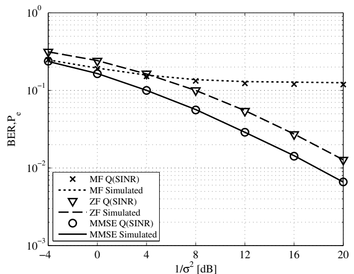
Fig. 4. Comparative BER and P_e for the MMSE, ZF and MF equalizers for the secondary (VFDM) system ( N = 64 , L = 16 , \alpha = 0 ).
