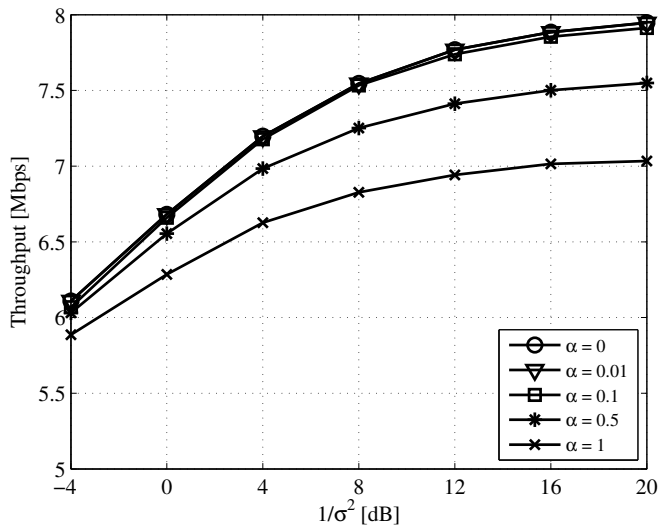
Fig. 8. Comparative throughput T for the MMSE equalizer for the secondary (VFDM) system with varying interference levels \alpha = \{0, 0.01, 0.1, 0.5, 1\} ( N = 64 , L = 16 ).
