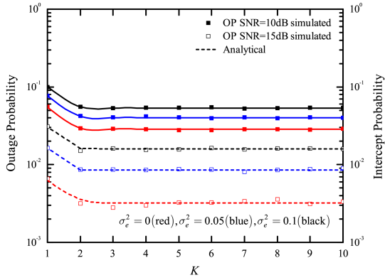
Fig. 4 OP versus K for difference \sigma_e^2 and SNR ( \alpha = 2, \mu = 0.8, \{\xi_1, \xi_2\} = \{0.06, 0.95\} and \kappa = 0.1 )
