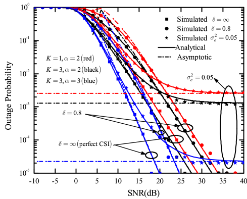
Fig. 11 OP versus SNR for different \alpha , K and \sigma_e^2 ( \mu = 0.8 , \{\xi_1, \xi_2\} = \{0.02, 0.99\} and \kappa = 0.1 )
