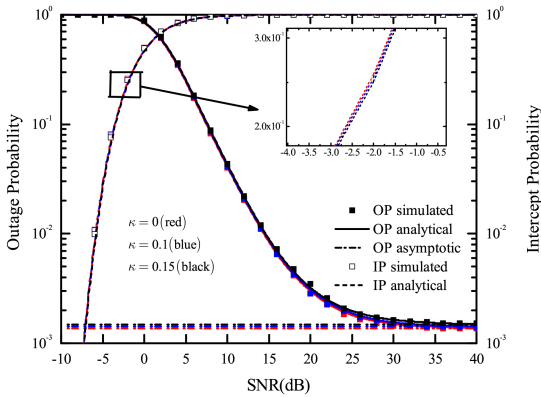
Fig. 6 Simulated OP and IP, analyse them versus SNR for different \kappa ( \alpha = 2, \mu = 0.8, \{\xi_1, \xi_2\} = \{0.06, 0.95\}, K = 2, N = 2 and \sigma_e^2 = 0.05 )
