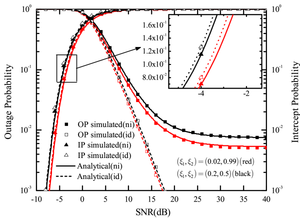
Fig. 3 OP and IP versus SNR for different \{\xi_1, \xi_2\} ( \alpha = 2 , \mu = 0.8 , \sigma_e^2 = 0.1 , \kappa = 0.15 , N = 2 and K = 2 )
