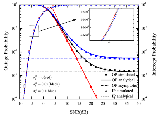
Fig. 8 OP and IP versus SNR for different \sigma_e^2 ( \alpha = 2, \mu = 0.8, \{\xi_1, \xi_2\} = \{0.06, 0.95\}, K = 2, N = 2 and \kappa = 0.1 )
