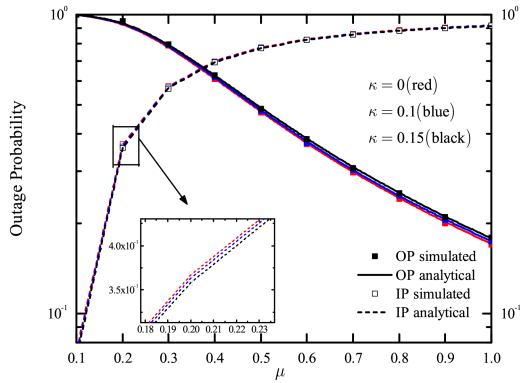
Fig. 2 OP and IP versus \mu for different \kappa ( \alpha = 2 , \{\xi_1, \xi_2\} = \{0.02, 0.99\} , SNR = 5 dB, \sigma_e^2 = 0.05 , N = 2 and K = 2 )
