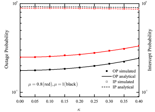
Fig. 7 OP and IP versus distortion noise parameter \kappa for different \mu ( \alpha = 2, \text{SNR} = 5 \text{ dB}, \{\xi_1, \xi_2\} = \{0.06, 0.95\}, K = 2, N = 2 and \sigma_e^2 = 0.05 )
