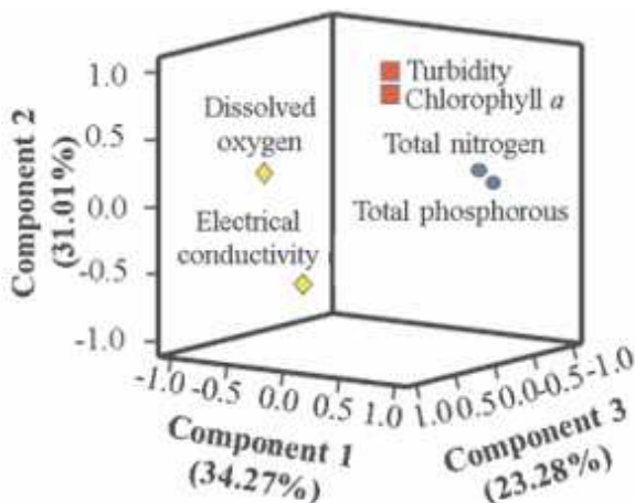
Figure 5 - PCA showing the variables explaining components 1, 2 and 3
