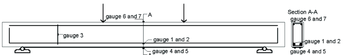
Figure 4 - Positioning of the strain gauges and of the transducers
