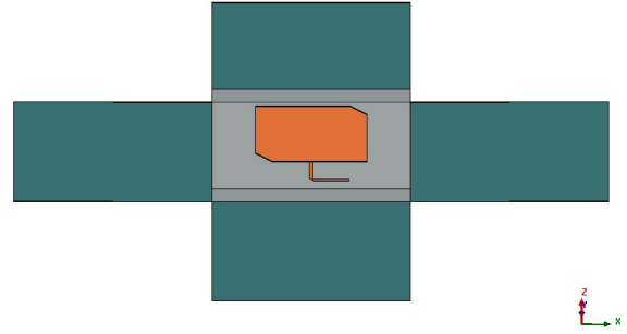
Fig. 2: Proposed antenna configuration.
