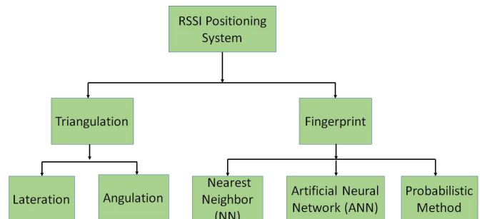
Fig. 1: Taxonomy of RSS positioning techniques in Wi-Fi.
