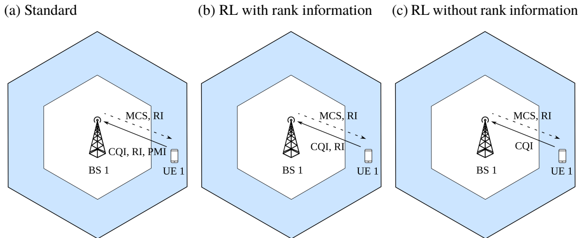
Figure 4.1 – Model of the signaling exchange
