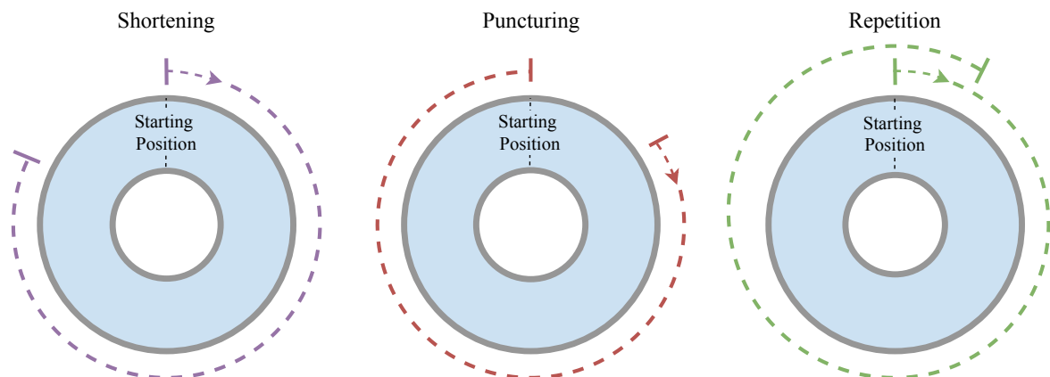
Figure 2.8 – Rate matching methods for polar coding
