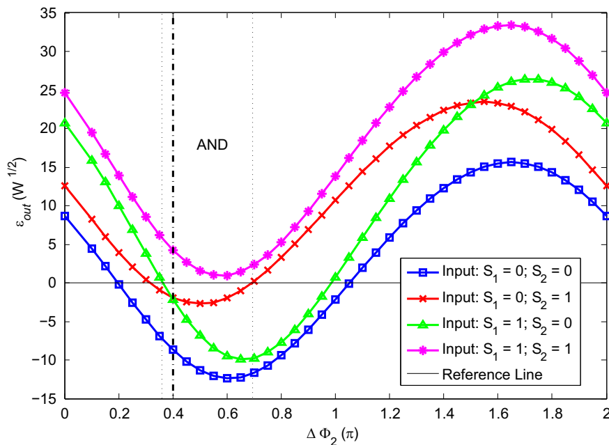
Fig. 6. Amplitude modulation \epsilon_{out}(W^{1/2}) measurement in the output S_4 , as a function of the phase shift \Delta\phi_2 \in [0, 2\pi] where \Delta\phi_1 = 0.642\pi and coupler length L = 1.1875 cm. The AND gate is observed in the interval [0.362\pi, 0.693\pi] . The AND gate obtained when \Delta\phi_2 = 0.4\pi is highlighted.
