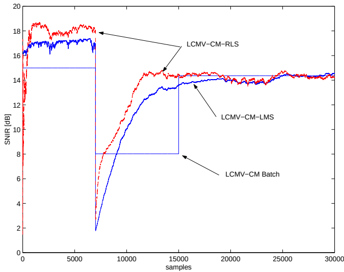
Fig. 5. Comparison between LCMV CM Batch Solution, LCMV CM -LMS and LCMV CM -RLS in a packet-like context.
