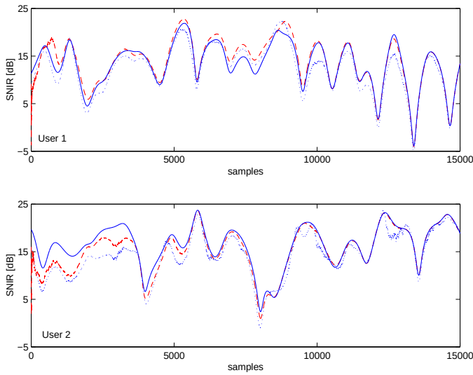
Fig. 4. Comparison between LCMV CM Batch Solution (solid lines), LCMV CM -LMS (dotted lines) and LCMV CM -RLS (dashed lines) for 100 km/h.
