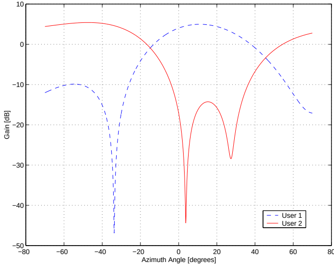
Fig. 2. Reception radiation pattern for LCMV CM method.
