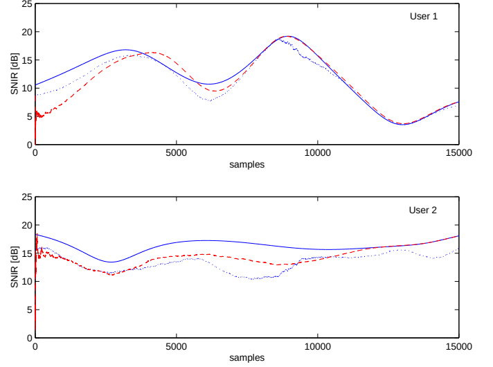
Fig. 3. Comparison between LCMV CM Batch Solution (solid lines), LCMV CM -LMS (dotted lines) and LCMV CM -RLS (dashed lines) for 15 km/h.
