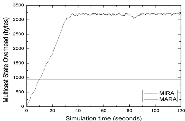
Fig. 6. Multicast state behaviour
