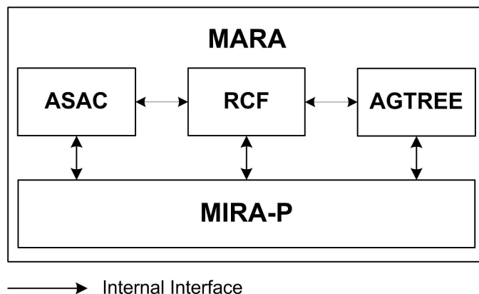
Fig. 1. Architecture of MARA
