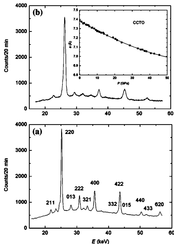
FIG. 3. Energy-dispersive diffraction patterns of \text{CaCu}_3\text{Ti}_4\text{O}_{12} recorded at (a) 4.0 GPa and (b) 24.0 GPa. The inset to panel (b) stands for the pressure-volume compression data of \text{CaCu}_3\text{Ti}_4\text{O}_{12} . The curve through the experimental points has been calculated from the Birch's equation [see Eq. (1)].
