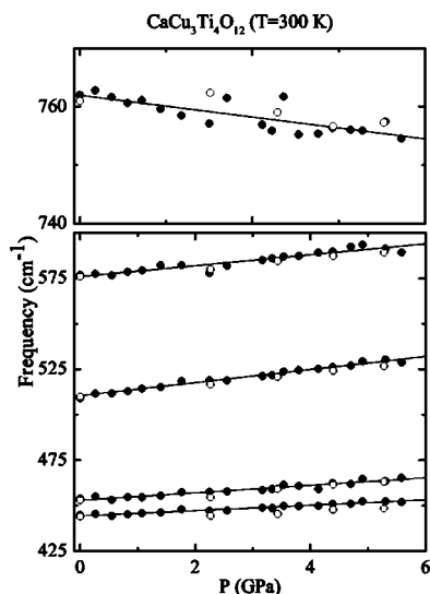
FIG. 2. Frequency vs pressure plots for CCTO Raman modes. The solid and open circles stand for compression and decompression runs, respectively. The error bar for both frequency ( \pm 1.5 \text{ cm}^{-1} ) and pressure ( \pm 0.1 \text{ GPa} ) are smaller than the symbols. The solid lines are fit to the experimental data using \omega(P) = \omega_0 + \alpha P .
