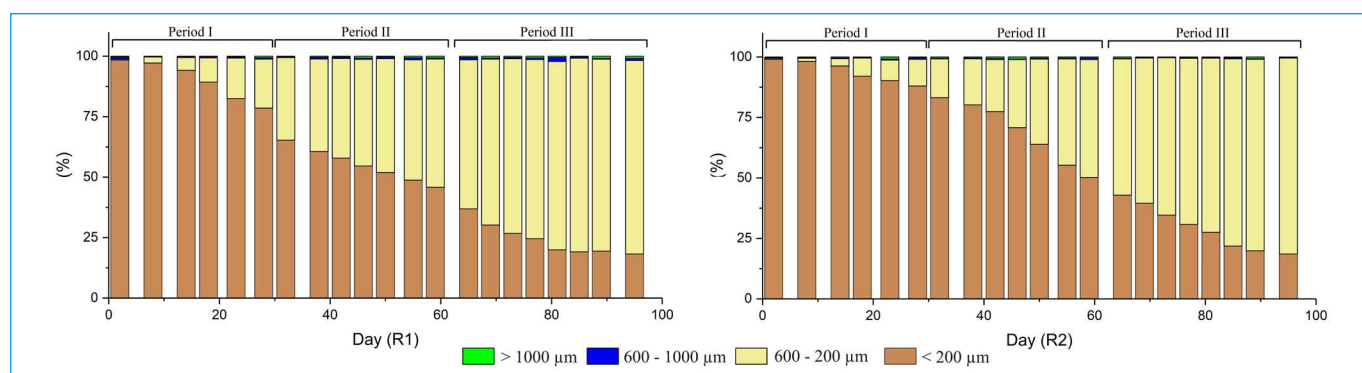
Figure 3 - Granule size distribution (% mass) in aerobic granular sludge systems.
