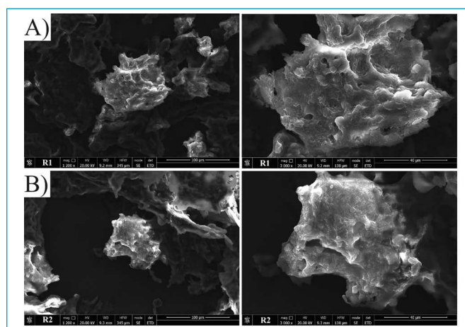
Figure 4 - Granule scanning electron micrograph of the reactors R1 (A) and R2 (B) at the end of Period III accurate to 1200\times (left side) and 3000\times (right side).
