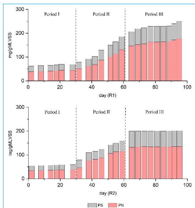
Figure 5 - Average quantification of extracellular polymeric substances.
