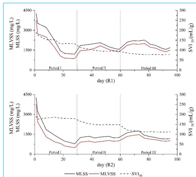
Figure 2 – Stability in terms of solids and SVI_{30} of aerobic granular sludge systems with 25% (R1) and 50% (R2) leachate with feeding and settling time of 20 min (Period I), feeding time of 40 min, and settling time of 10 min (Period II) and with increased dissolved oxygen concentration (Period III).
