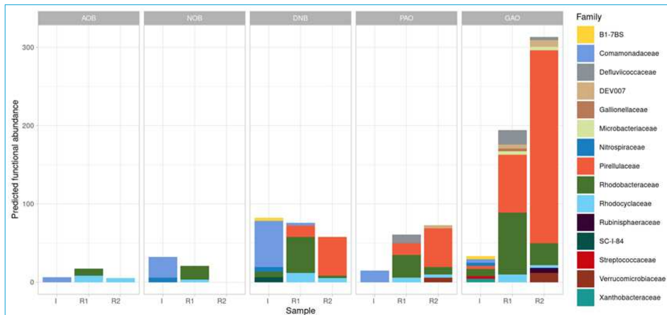
Figure 7 – Functional taxonomic classification distribution at the experiment's end.
