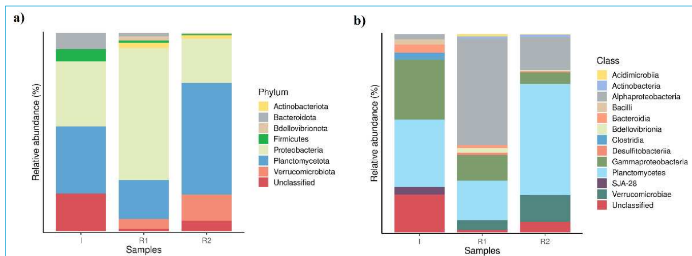
Figure 6 - Bacterial community structure at the phylum (a) and class (b) level of the two reactors and the inoculum (I).
