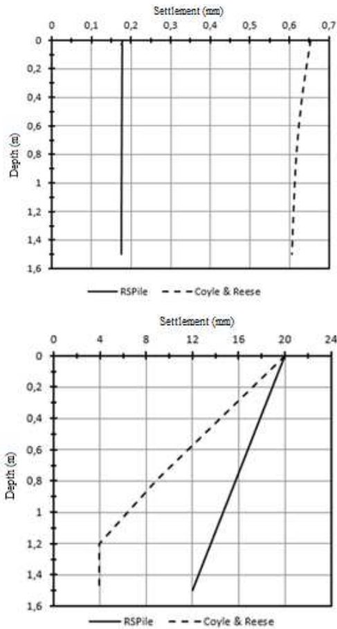
Figure 14 Estimation of load transfer for workload: displacement profile and load-depth diagram
