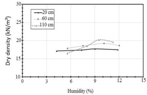
Figure 4 Compaction curves
