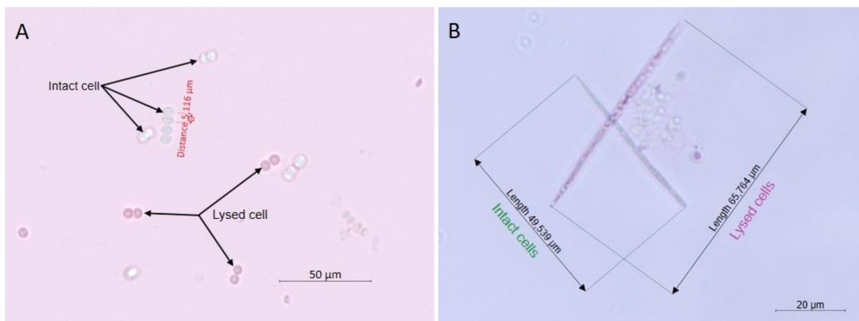
Fig. 1. D. circinale (A) and R. raciborskii (B) organisms intact and with compromised integrity (pink color).
