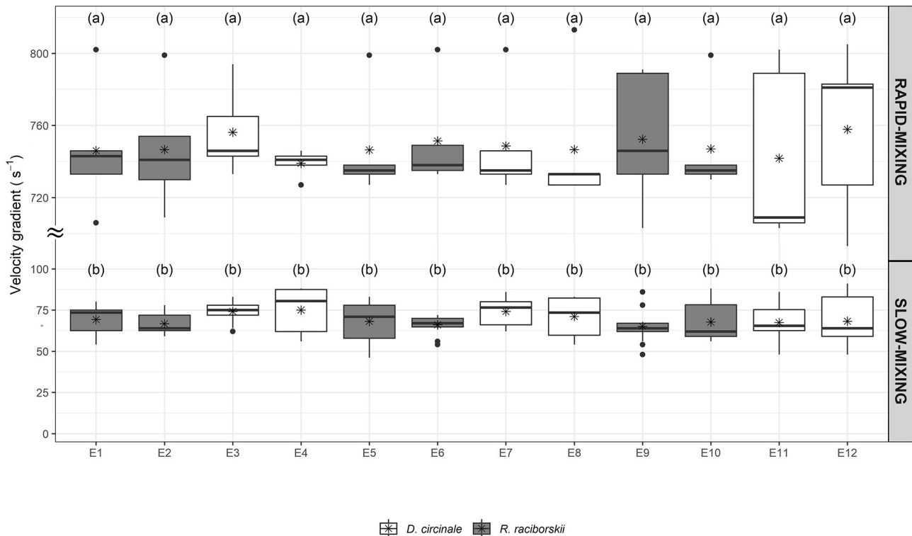
Fig. 2. Velocity gradients for rapid-mixing and slow-mixing. The dots represent outliers, the asterisks represent means and different letters mean significant statistical differences ( p < 0.05 ).
