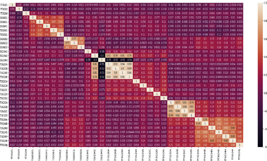
Graph 1. Pearson's Correlation
