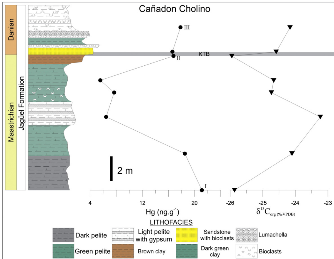
Fig. 9. Hg and δ 13 C org variation curves across the KTB at the Cañadon Cholino section.
