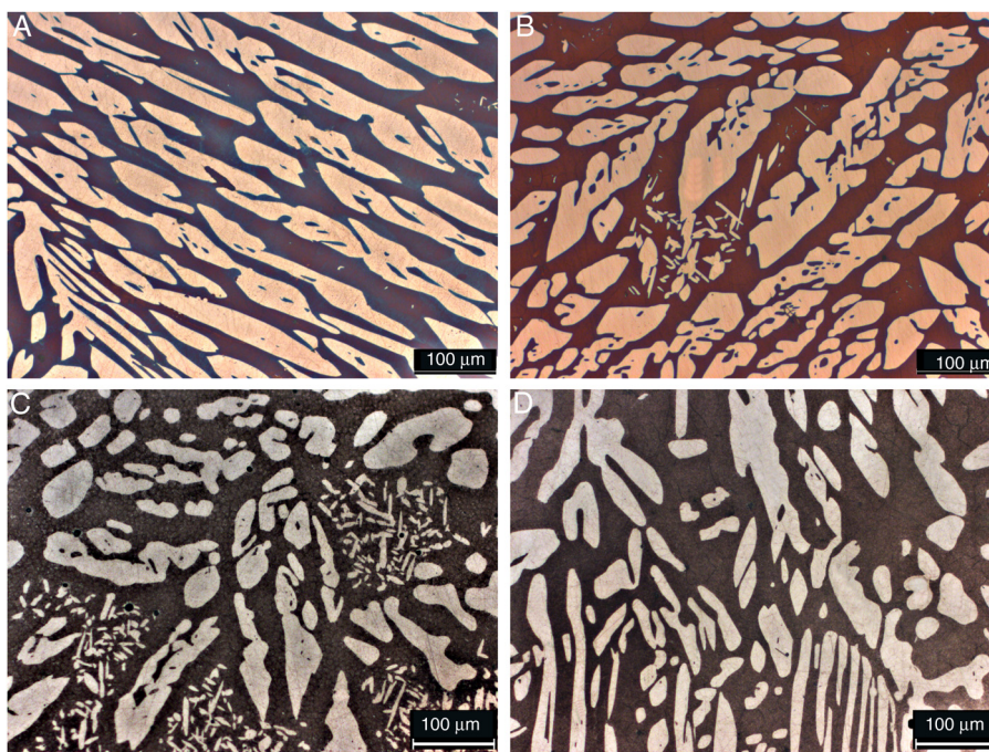
Fig. 1 – Optical micrographs of the microstructures of samples (A) 1B annealed, (B) 1B aged at 600 °C for 1 h, (C) 3A annealed and (D) 3A aged at 600 °C for 1 h.
