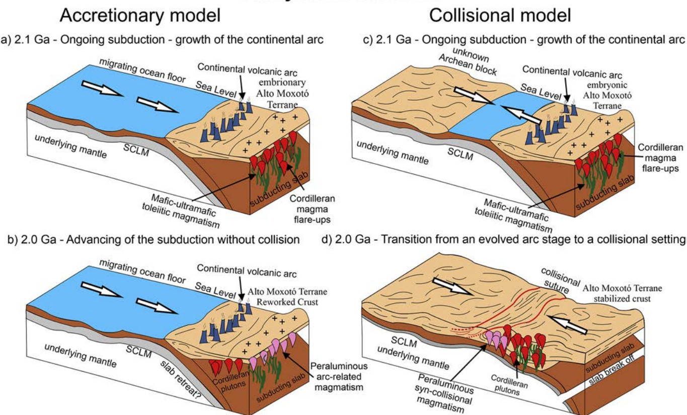
Fig. 10. Possible tectonic scenarios for the Alto Moxotó Terrane evolution based on this study.
