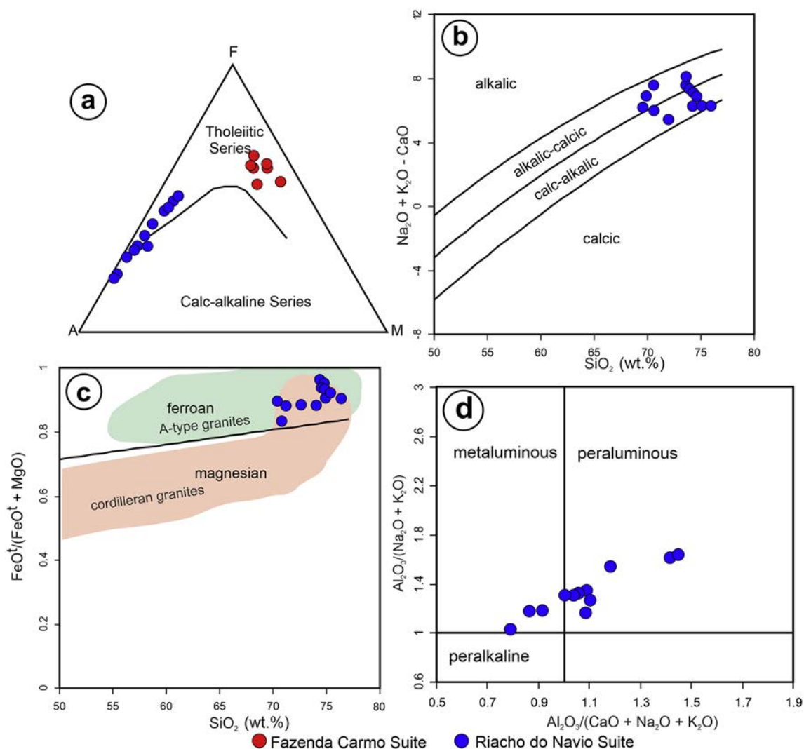
Fig. 7. Geochemical characteristics of the Fazenda Carmo and Riacho do Navio Suites. (a) AFM diagram from Irvine and Baragar (1971); (b) \text{SiO}_2 vs. \text{Na}_2\text{O} + \text{K}_2\text{O} - \text{CaO} diagram from Frost et al. (2001); (c) \text{SiO}_2 vs. \text{FeO}^t/(\text{FeO}^t + \text{MgO}) diagram from Frost et al. (2001); (d) A/CNK diagram molar diagram from Maniar and Piccoli (1989).
