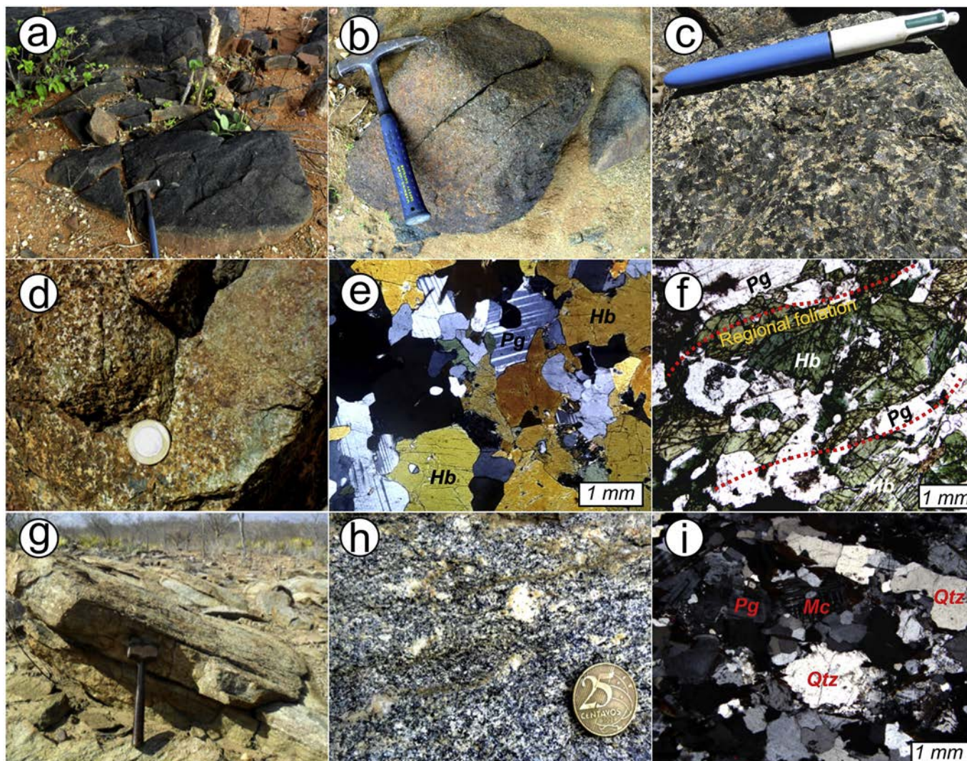
Fig. 3. Field aspects of the studied units. Fazenda Carmo Suite: (a) slightly foliated boulder of amphibolite; (b) block of garnet-bearing amphibolite; (c) coarse-grained metagabbro; (d) metapyroxenite boulder exhibiting green-colored alteration minerals; (e) granoblastic texture on less deformed amphibolite; (f) amphibolite exhibiting elongated hornblende crystals along foliation planes imposed by the regional deformation. Riacho do Navio Suite: (g) gentle-dipping sheet of metagranitic rock due to thrust tectonics; (h) augen-gneiss facies exhibiting deformed K-feldspar porphyroclast; (i) recrystallized fabric of orthogneiss exhibiting intense quartz recrystallization, including ribbon-like crystals. Hb–hornblende, Pg–plagioclase, Mc–microcline, Qtz–quartz.
