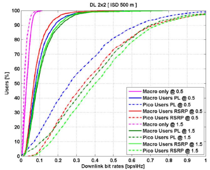
Fig. 8. Downlink bit rates by varying the building position compared with the reference case.
