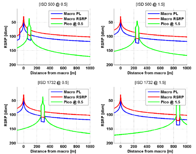
Fig. 3. Pathloss analysis for pico coverage area at different positions with two ISD systems.
