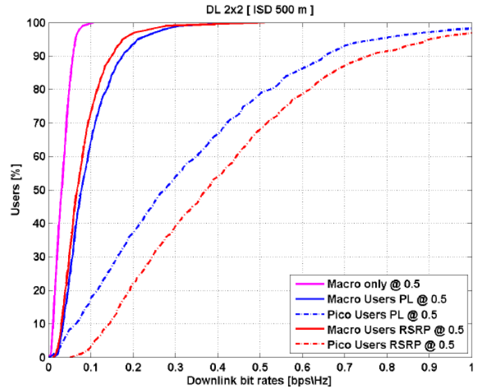
Fig. 5. Downlink bit rates for the reference case.
