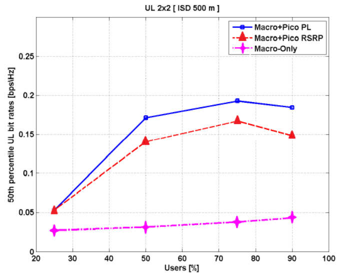
Fig. 11. 50 th percentile of uplink bit rates for different systems and hotspot densities.
