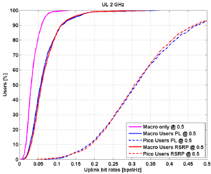
Fig. 6. Uplink bit rates for the reference case.
