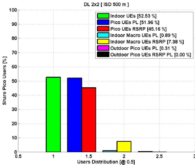
Fig. 4. Users distribution for the reference case.
