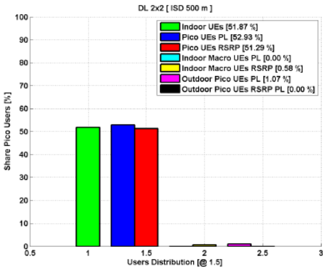
Fig. 7. Users distribution by varying the building position @ 1.5 times macro radius.
