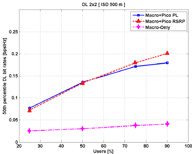
Fig. 10. 50 th percentile of downlink bit rates for different systems and hotspot densities.
