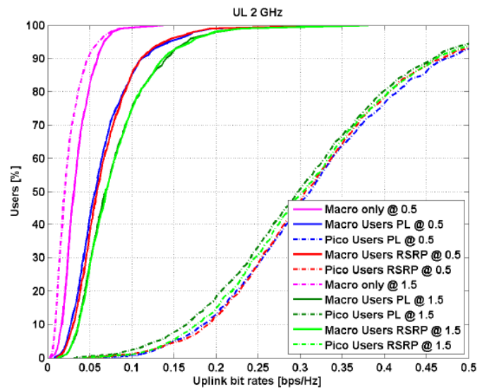
Fig. 9. Uplink bit rates by varying the building position compared with the reference case.
