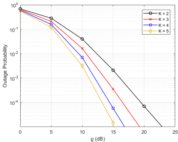
Fig. 7. Outage probability versus \rho for incremental relaying considering OR scheme and different number of relays.
