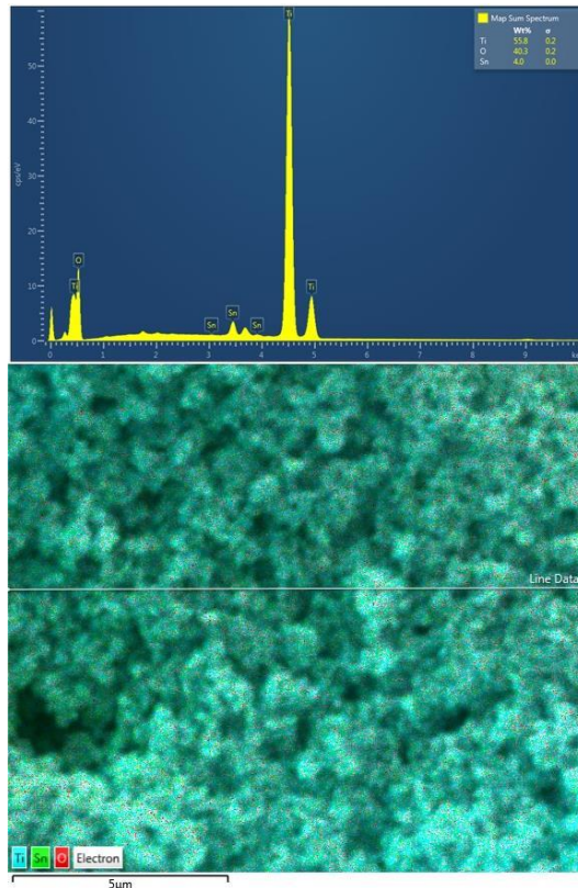
Figure 3: EDS from sample 450 with the respective mapping area.
