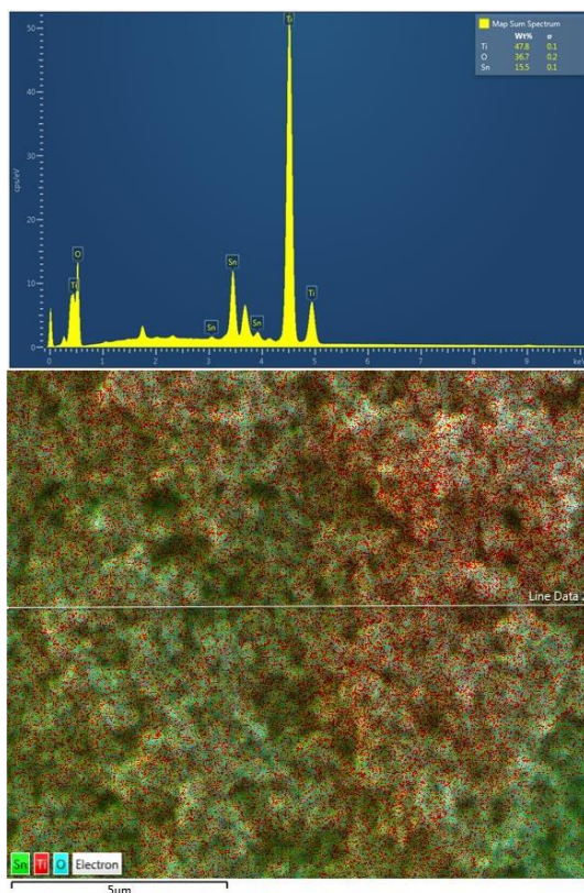
Figure 5: EDS of sample 600 with the respective mapping area.
