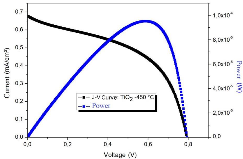
Figure 8: J-V curve of sample 450.
