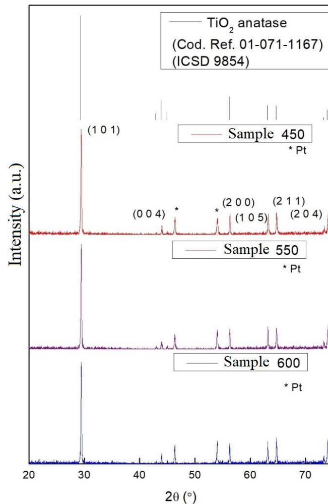
Figure 6: X-ray diffractograms of TiO 2 samples.
