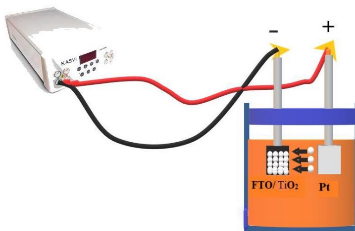
Figure 1: Illustration of the electrophoretic deposition.
