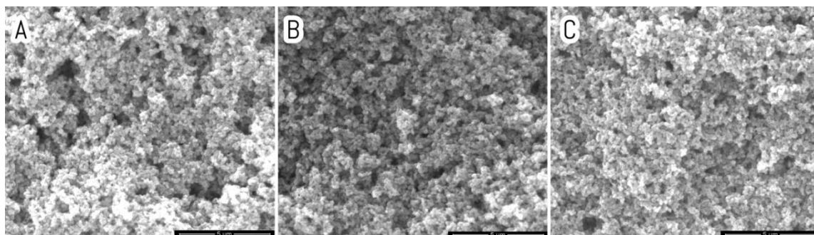
Figure 2: SEM images of TiO 2 film surfaces for sintering temperature of 450 °C (A), 550 °C (B) and 600 °C (C).
