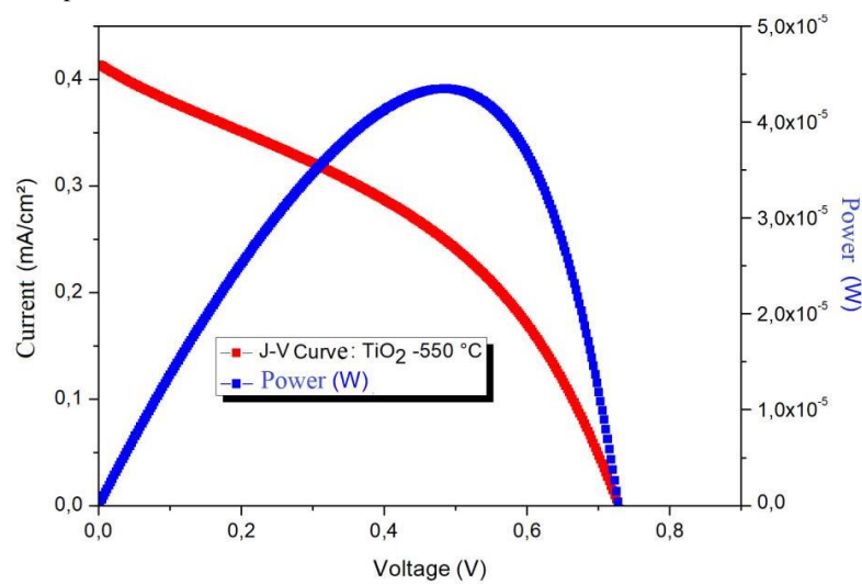
Figure 9: J-V curve of sample 550.
