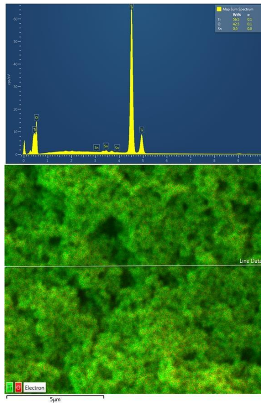
Figure 4: EDS of sample 550 with the respective mapping area.
