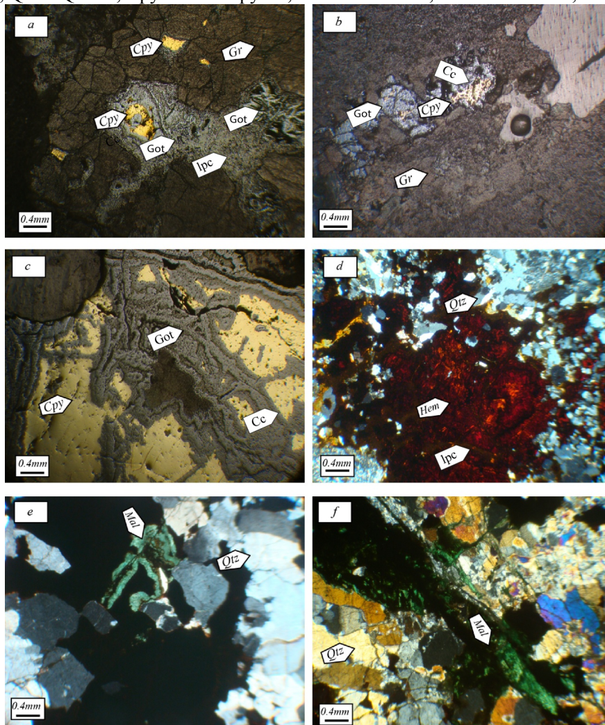
Figura 10 - (a): Chalcopyrite, which has altered to Chalcocite from the margin, and goitaite (b) Chalcopyrite alteration to Chalcocite and goitaite (c): The greater the amount of chalcopyrite with increasing depth and the alteration of the mineral to the Chalcocite and goitaite from the margin, (d): Hematite resulted from iron sulfide minerals alteration (e): Malachite and quartz in the vein zone (f): Malachite placement in the final stages of alteration in the vein section with green color Gr = Garnet, Qtz = Quartz, Cpy = Chalcopyrite, Cc = Chalcocite, Hem = Himatite, Mal = Malachite
