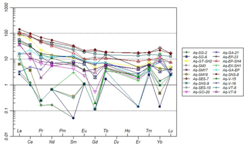
Figure 11 - Spider diagrams of samples in different zones of AghBolagh cooper deposit normalized to Chondrite
