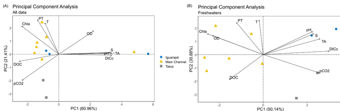
Fig. 7. Principal Component Analysis using all sampling points (a) and only in freshwater stations (b). Main channel stations are represented in yellow triangles, Tatus channel in gray squares and Igarapé dos Periquitos channel in blue dots.
