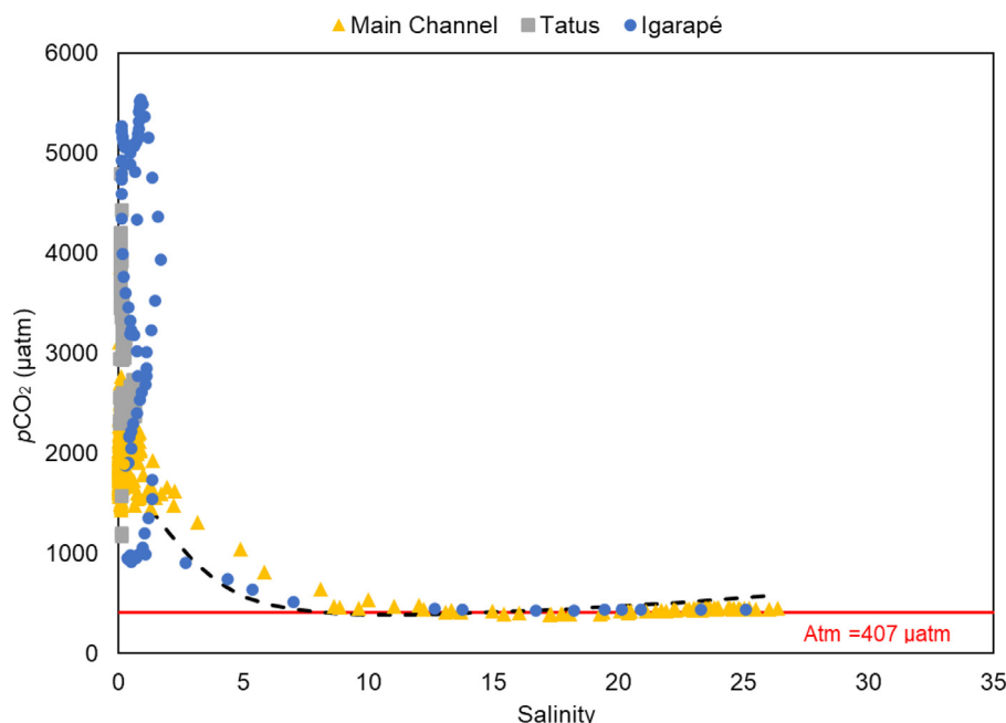
Fig. 4. Distribution of surface water p\text{CO}_2 against salinity. Different colors indicate the different channels sampled (yellow triangle — main channel; gray square — Tatus channel; blue circle — Igarapé dos Periquitos). Dashed black line indicates conservative mixing. Solid red line represents atmospheric value.
