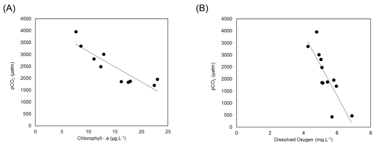
Fig. 6. (a) Estuarine pCO 2 against Chl- a in freshwaters ( S < 1 ) stations. Spearman correlation coefficient r = -0.80 ( p < 0.01 ). (b) Estuarine pCO 2 against DO in all stations. Spearman correlation coefficient r = -0.85 ( p < 0.01 ).
