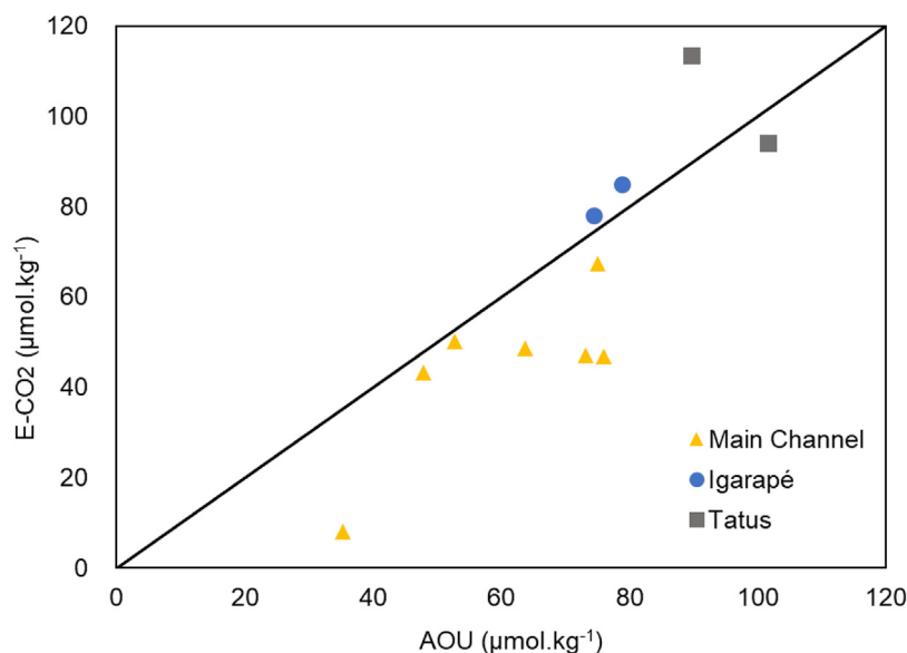
Fig. 5. Excess \text{CO}_2 vs. Apparent Use of Oxygen in the Parnaíba river estuary, for the channels sampled (yellow triangles = main channel; blue circles = mangrove channel (Igarapé dos Periquitos); and gray squares = Tatus channel). The 1:1 line represents the quotient between \text{CO}_2 and \text{O}_2 during the processes of photosynthesis and respiration.
