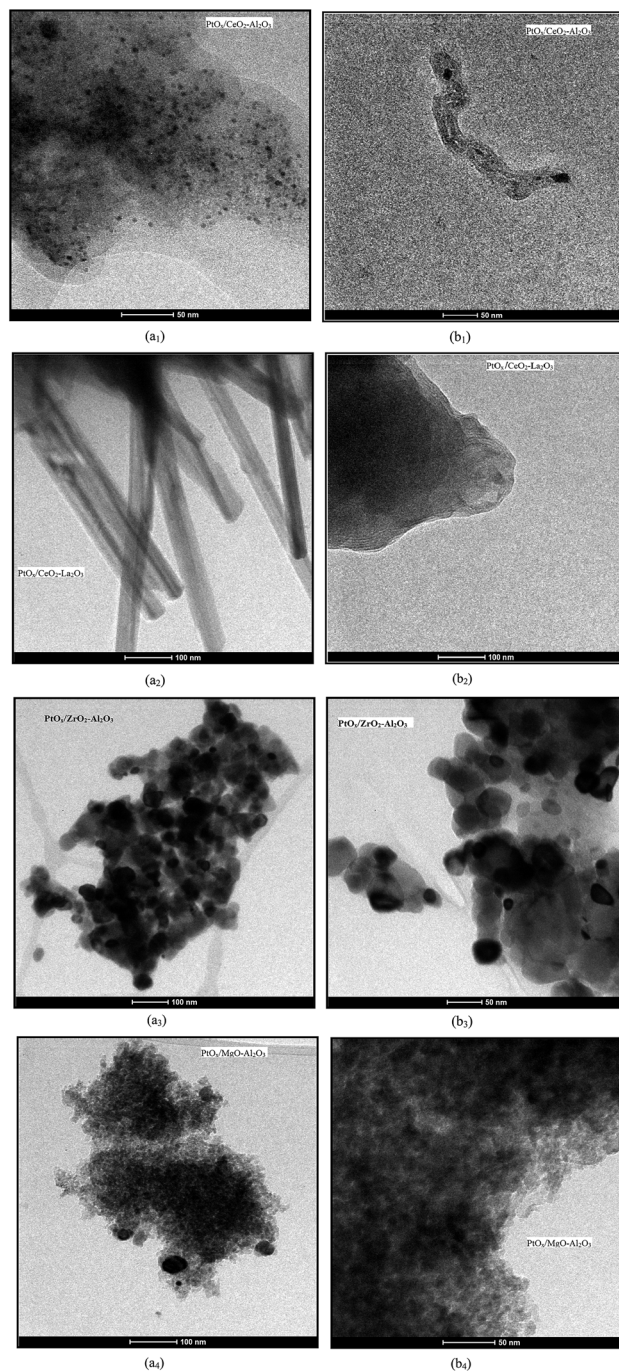
Fig. 4 (a) TEM and HRTEM images of the spent catalysts, after 5 h on stream in steam reforming of glycerol and water to glycerol molar ratio of 9 at 600^\circ\text{C} .
